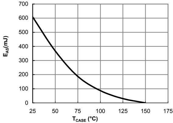
Figure 12: Avalanche energy
