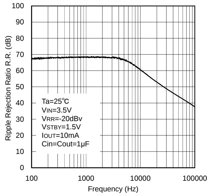
Figure 59. Ripple Rejection Ratio vs. Frequency
