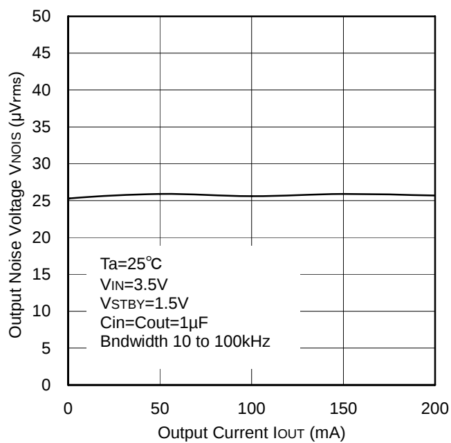
Figure 15. Output Noise Voltage vs. Output Current
