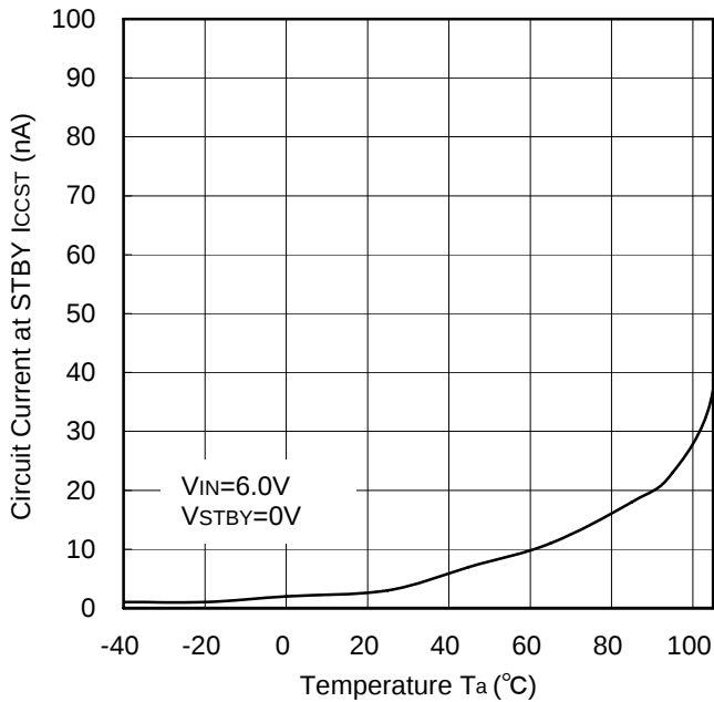
Figure 56. Circuit Current ( at STBY) vs. Temperature
