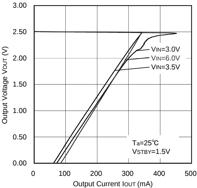
Figure 52. OCP Threshold
