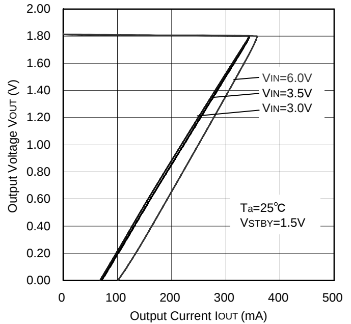
Figure 30. OCP Threshold
