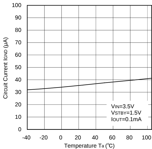
Figure 54. Circuit Current vs. Temperature
