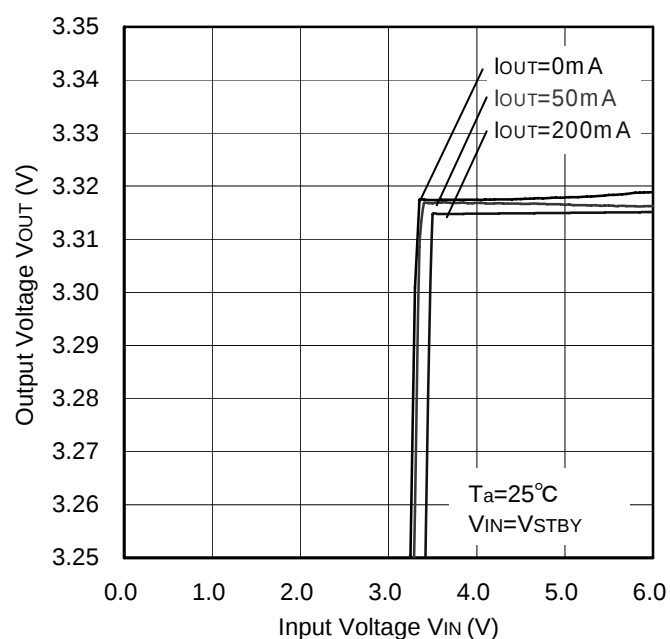
Figure 71. Line Regulation
