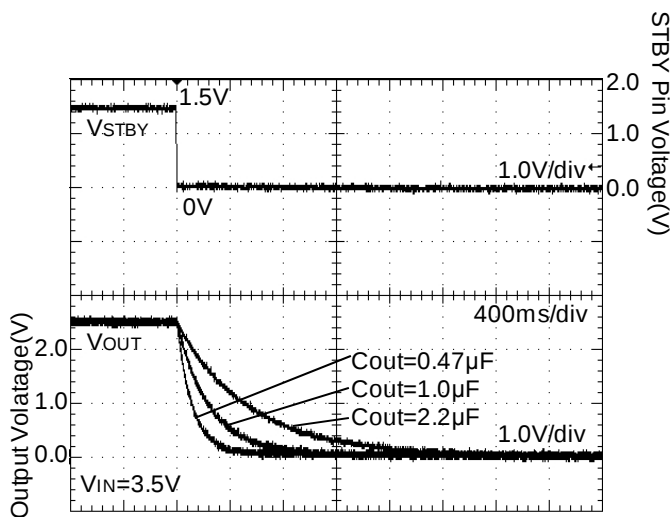
Figure 68. Discharge Time (ROUT=none)
