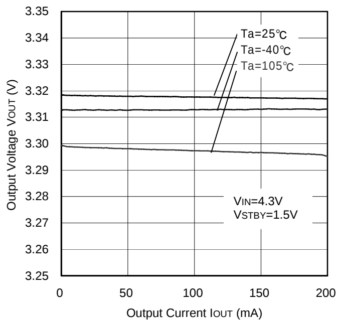
Figure 73. Load Regulation
