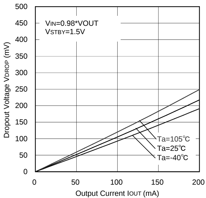
Figure 58. Dropout Voltage vs. Output Current
