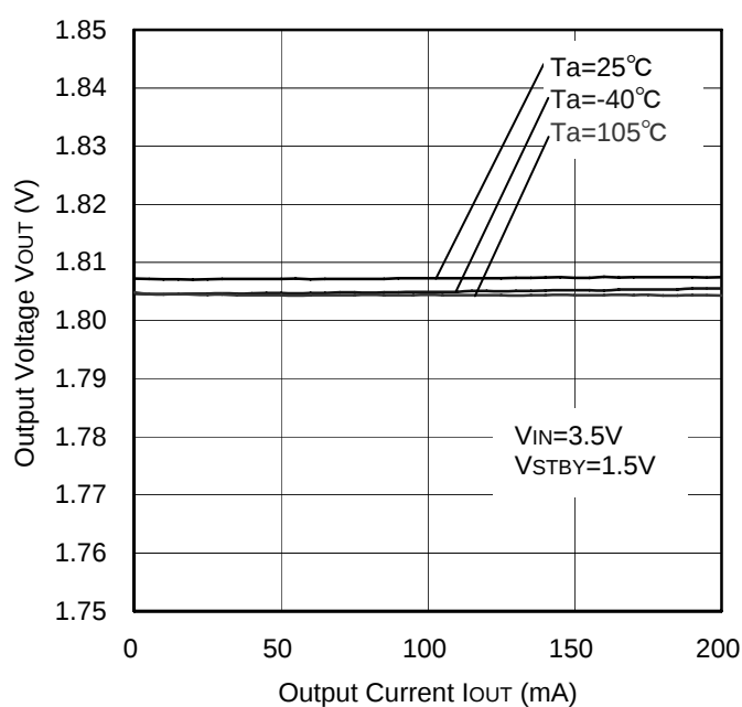
Figure 28. Load Regulation
