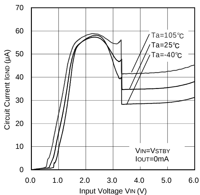
Figure 72. Circuit Current vs. Input Voltage
