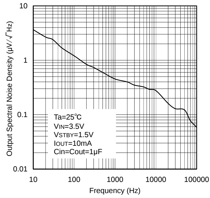
Figure 61. Output Spectral Noise Density vs. Frequency
