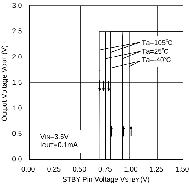
Figure 55. STBY Threshold
