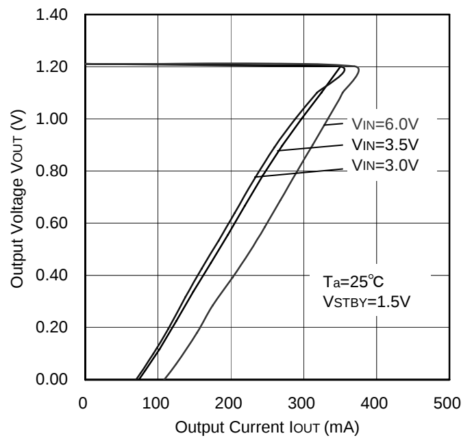
Figure 8. OCP Threshold
