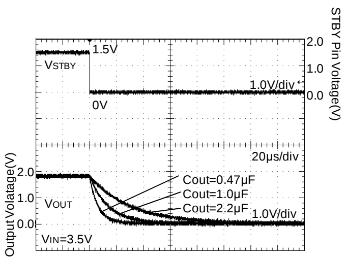
Figure 46. Discharge Time (ROUT=9Ω)
