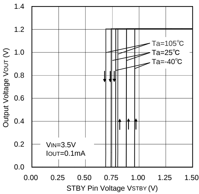
Figure 11. STBY Threshold
