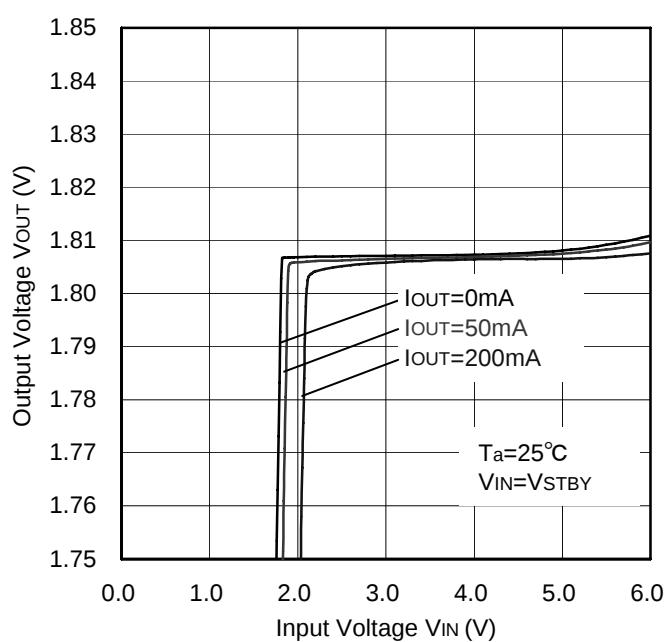
Figure 26. Line Regulation
