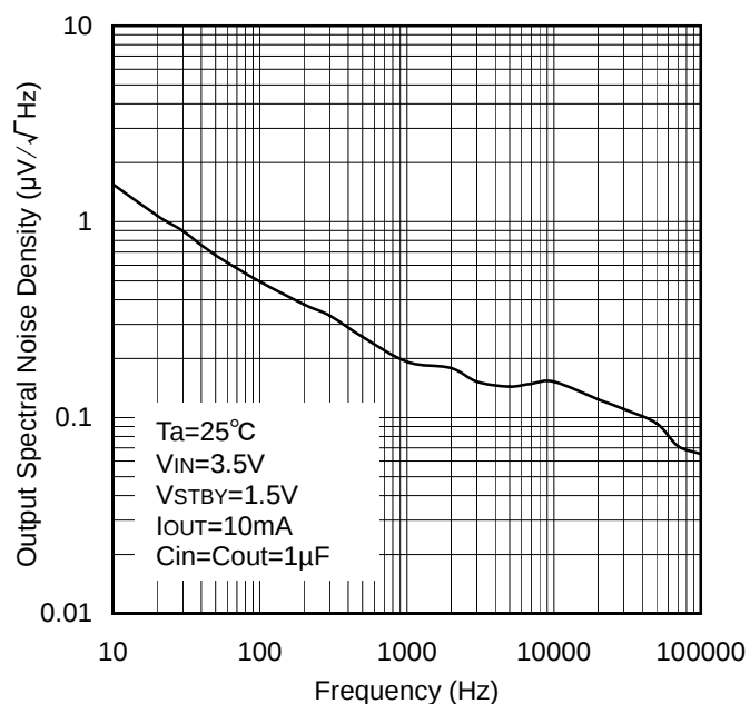
Figure 16. Output Spectral Noise Density vs. Frequency
