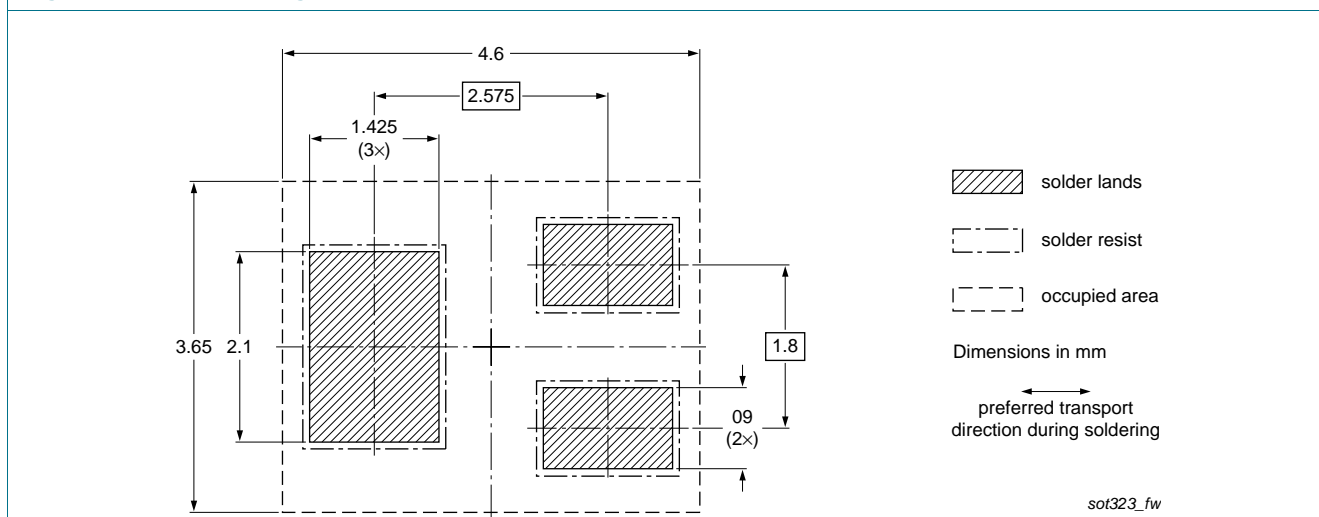
Fig 20. Wave soldering footprint for SOT323 (SC-70)
