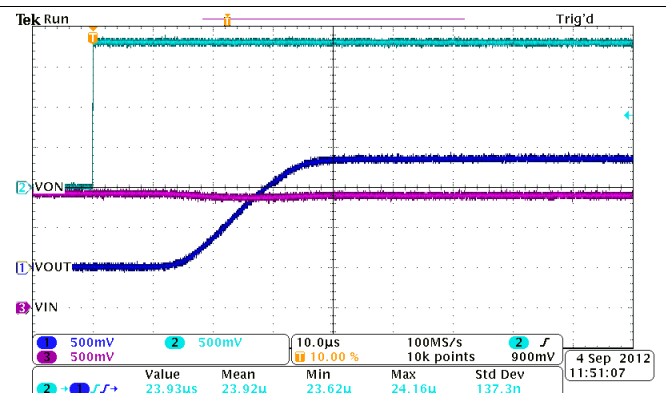
Figure 19. Turn-On Response Time (V_{IN} = 1.4\text{ V}, C_{IN} = 10\ \mu\text{F}, C_L = 1\ \mu\text{F}, R_L = 10\ \Omega)
