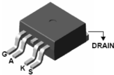
TO263 5 LEADS
