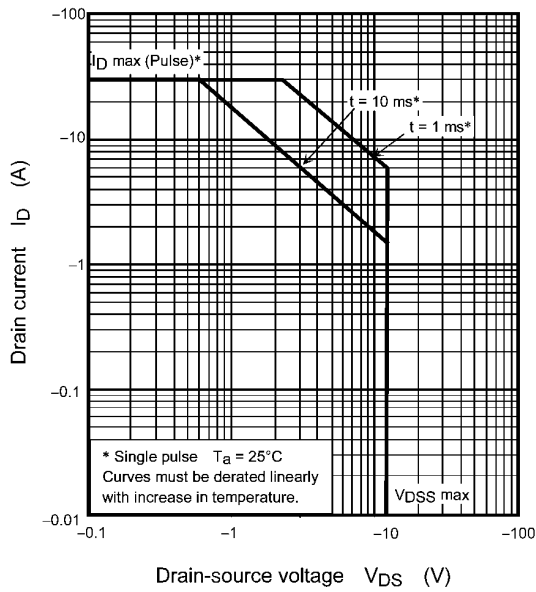
Fig. 8.15 Safe Operating Area
