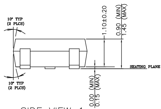
SIDE VIEW 1
