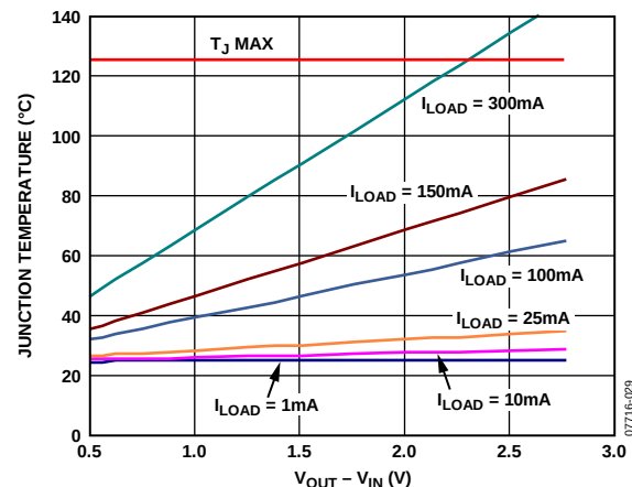
Figure 34. 100 mm 2 of PCB Copper, T_A = 25^\circ\text{C}
