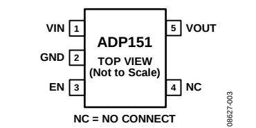
Figure 4. 5-Lead TSOT Pin Configuration
