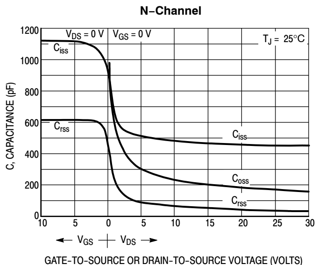
Figure 7. Capacitance Variation
