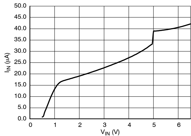
Figure 13. Supply Current vs. Input Voltage, 5.0 V version
