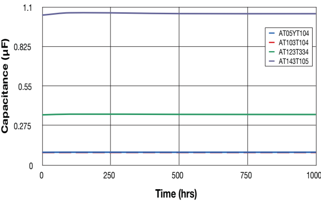
250°C Life Test @ 2x Rated Voltage (VHT Dielectric)
