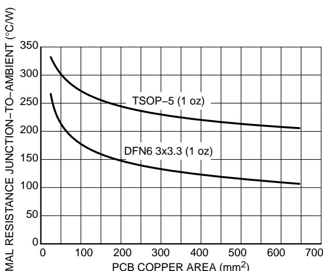
Figure 34. R thJA vs. PCB Copper Area
