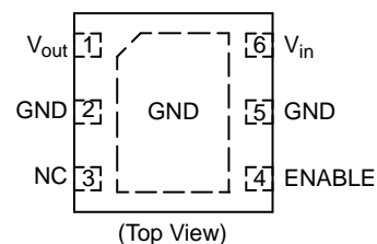
Figure 4. DFN6 (2x2.2)
