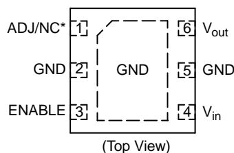
Figure 3. DFN6 (3x3)
