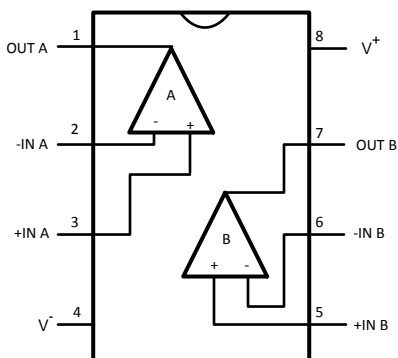
Figure 2. SOIC-8/MSOP-8 (LMH6658)
