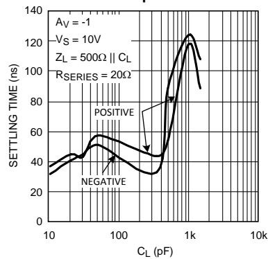
0.1% Settling Time vs. Cap Load
