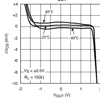
ΔV OS vs. V OUT
