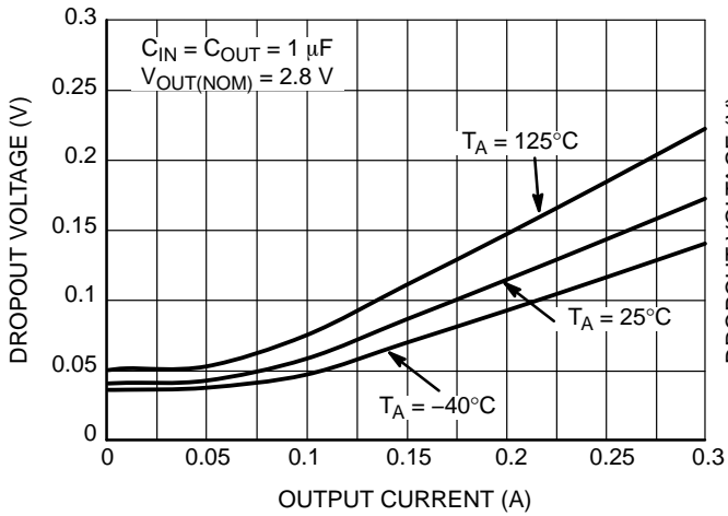
Figure 20. Dropout Voltage vs. Output Current V_{OUT} = 2.8 V
