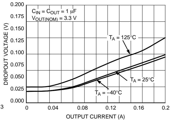
Figure 23. Dropout Voltage vs. Output Current V_{OUT} = 3.3 V
