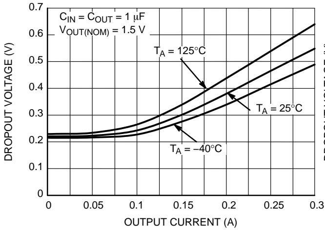
Figure 18. Dropout Voltage vs. Output Current V_{OUT} = 1.5 V
