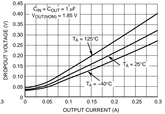
Figure 19. Dropout Voltage vs. Output Current V_{OUT} = 1.85 V
