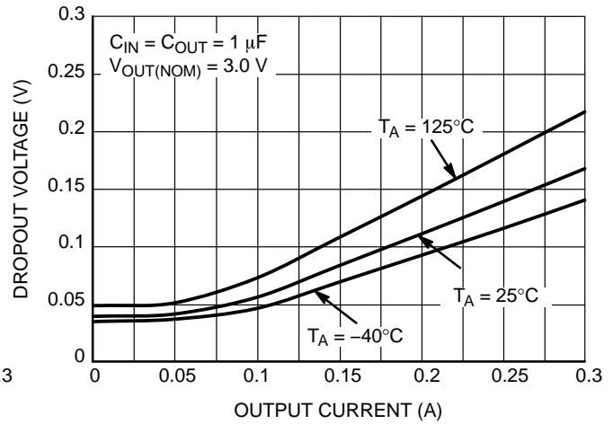
Figure 21. Dropout Voltage vs. Output Current V_{OUT} = 3.0 V
