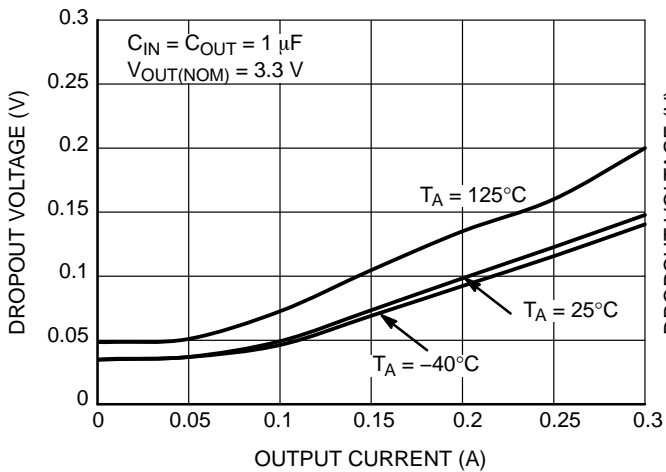
Figure 22. Dropout Voltage vs. Output Current V_{OUT} = 3.1 V
