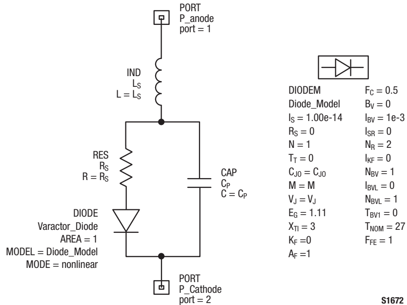
Figure 3. SPICE Model
