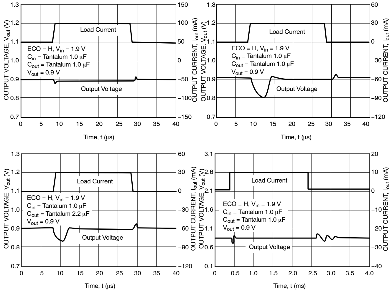
Figure 29. Load Transient Response
