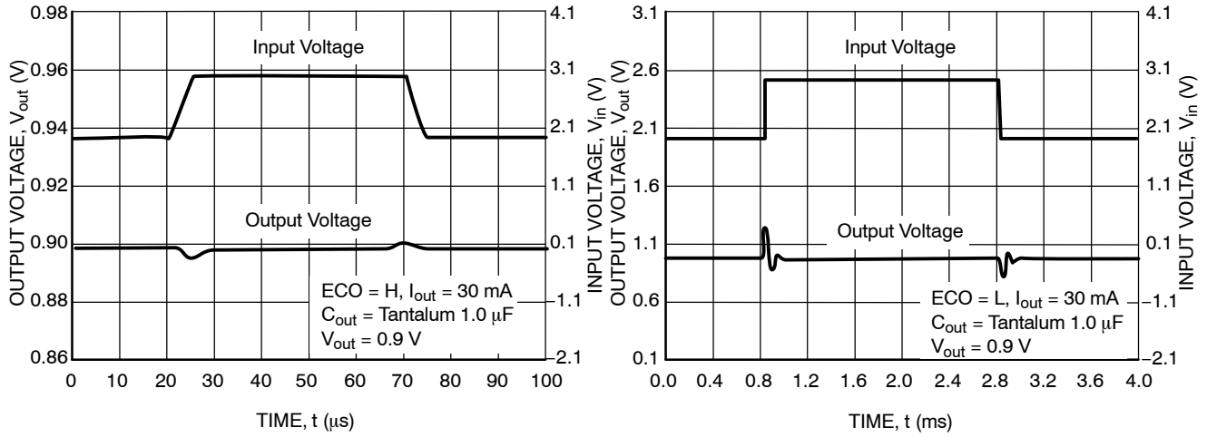
Figure 28. Input Transient Response
