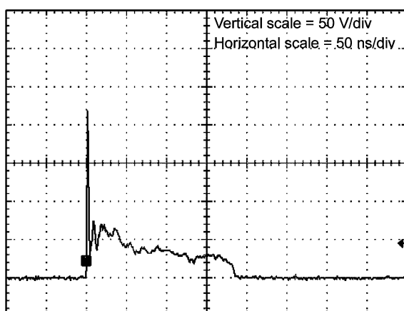
Fig. 11.1 +8 kV (I/O to GND)
