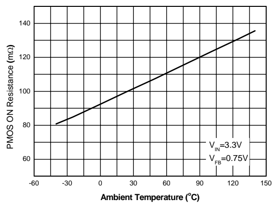
Figure 7. PMOS ON Resistance vs. Ambient Temperature
