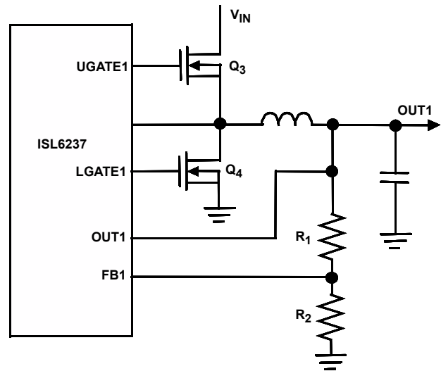
FIGURE 72. SETTING V OUT1 WITH A RESISTOR DIVIDER
