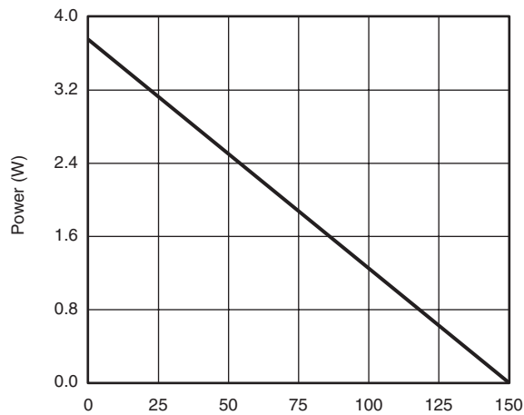
T_C - Case Temperature ( ^\circ\text{C} )
