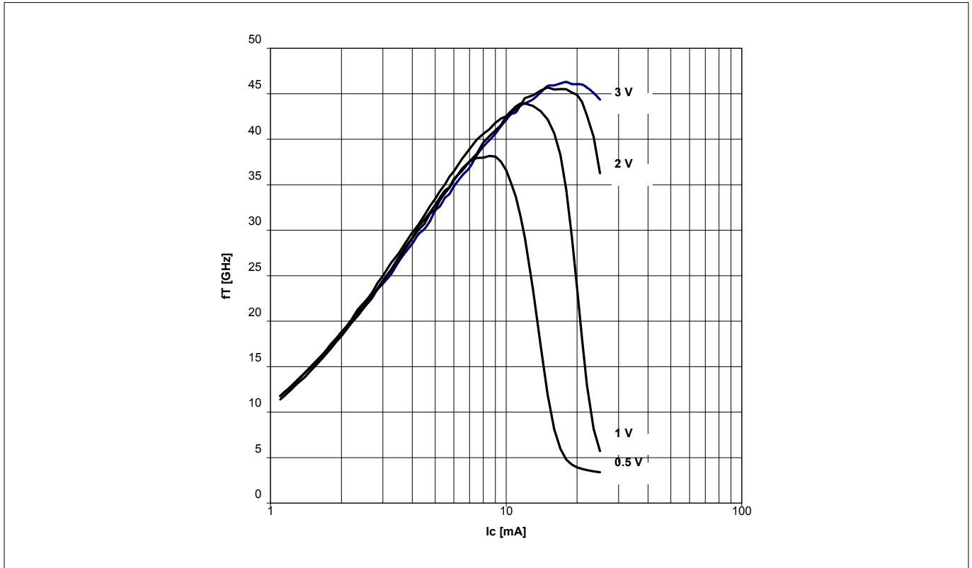
Figure 5 Transition frequency f_T = f(I_C, V_{CE}) , f = 1 \text{ GHz} , V_{CE} = \text{parameter}
