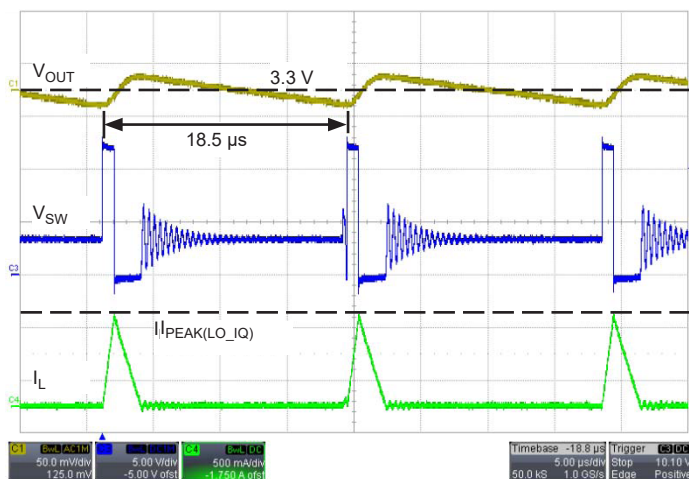
Figure 4: Low-IQ PFM Mode Operation at V_{\text{IN}} = 12 V, V_{\text{OUT}} = 3.3 V, and I_{\text{OUT}} = 66 mA.
