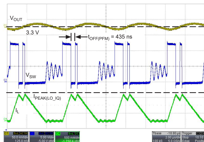
Figure 5: Low-IQ PFM Mode Operation at V_{\text{IN}} = 12 V, V_{\text{OUT}} = 3.3 V, and I_{\text{OUT}} = 330 mA.
