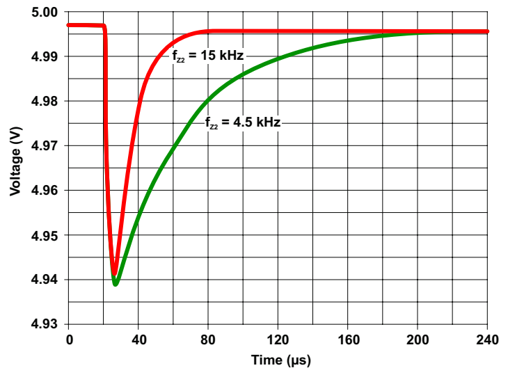
Figure 23: Transient Recovery Comparison for f_{Z2} at 4.5 kHz/63° and 15 kHz/51°.
