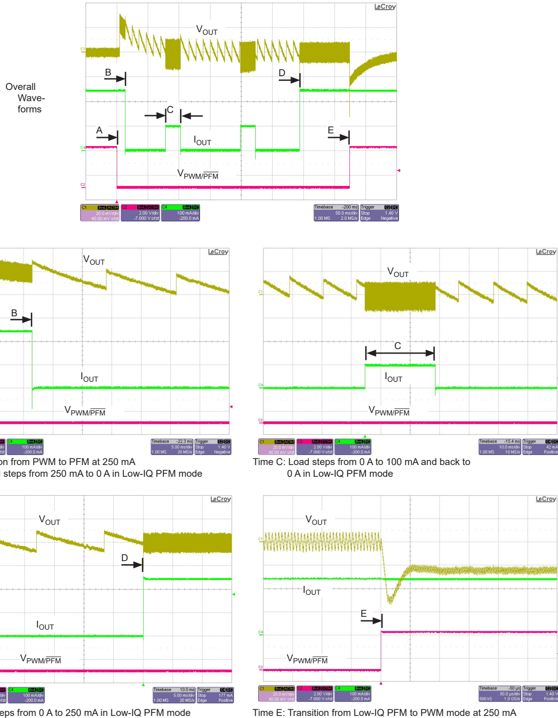
Figure 6: Transitions between PWM Mode and Low-IQ PFM Mode, and Load Transient Responses
