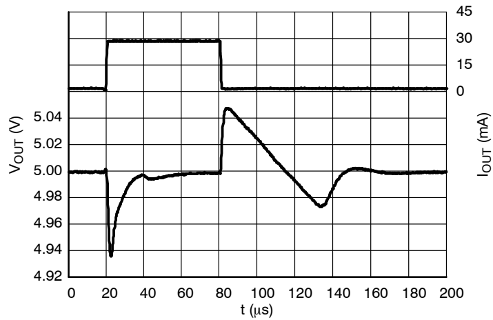
Figure 30. Load Transients, 5.0 V Version, I_{OUT} = 1 - 30 \text{ mA} , t_R = t_F = 0.5 \mu s , V_{IN} = 6.0 \text{ V}
