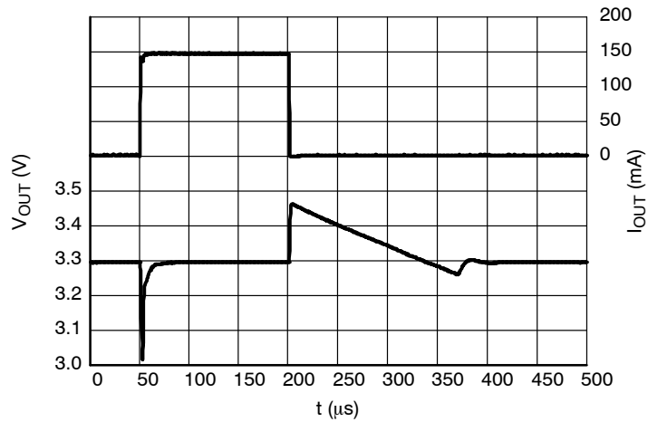
Figure 32. Load Transients, 3.3 V Version, I_{OUT} = 1 - 150 \text{ mA} , t_R = t_F = 0.5 \mu s , V_{IN} = 3.8 \text{ V}
