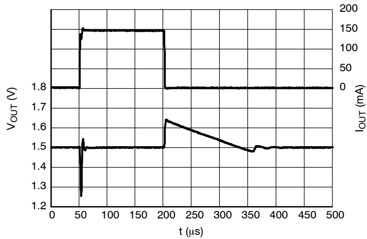
Figure 31. Load Transients, 1.5 V Version, I_{OUT} = 1 - 150 \text{ mA} , t_R = t_F = 0.5 \mu s , V_{IN} = 2.6 \text{ V}
