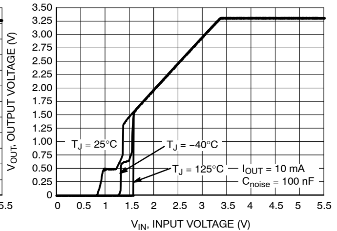
Figure 46. Output Voltage vs. Input Voltage, V_{OUT} = 3.3\text{ V} , C_{OUT} = 1\ \mu\text{F}
