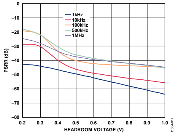
Figure 17. PSRR vs. Headroom Voltage at Various Frequencies, I_{LOAD} = 200 mA
