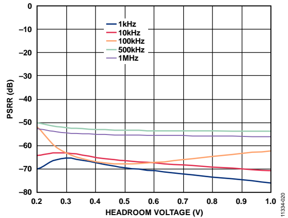
Figure 20. PSRR vs. Headroom Voltage at Various Frequencies, I_{LOAD} = 10 mA
