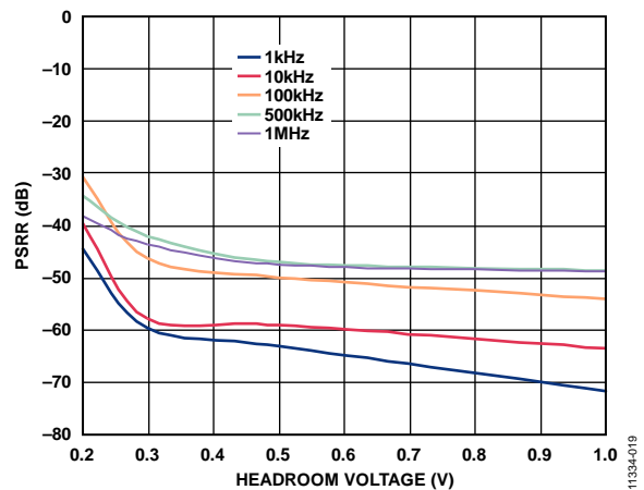
Figure 19. PSRR vs. Headroom Voltage at Various Frequencies, I_{LOAD} = 50 mA
