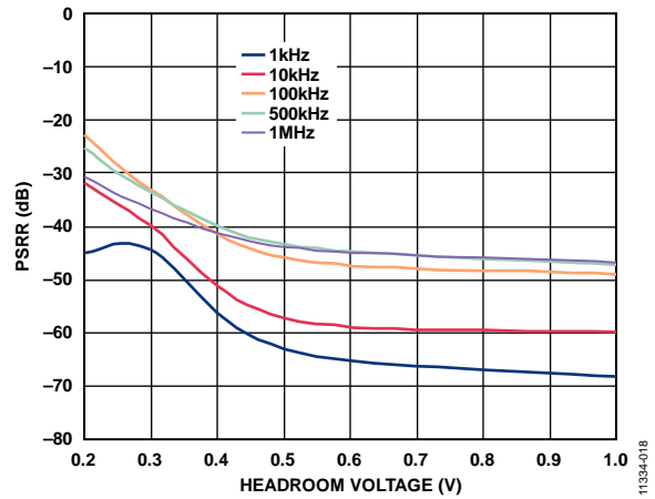
Figure 18. PSRR vs. Headroom Voltage at Various Frequencies, I_{LOAD} = 100 mA
