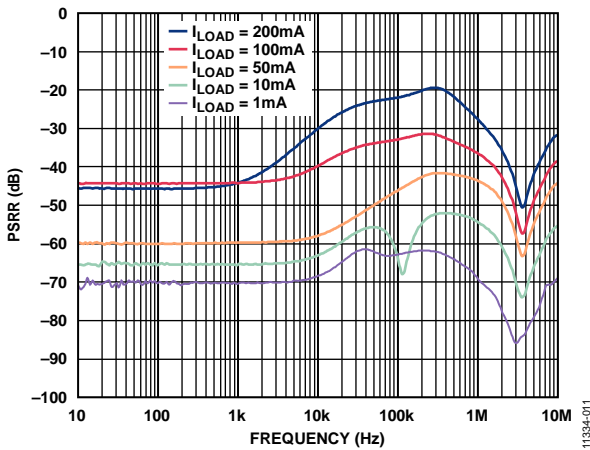
Figure 16. PSRR vs. Frequency and Load Current, 300 mV Headroom, V_{OUT} = 2.5 V
