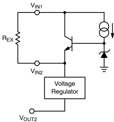
Figure 42. Power Shunt
