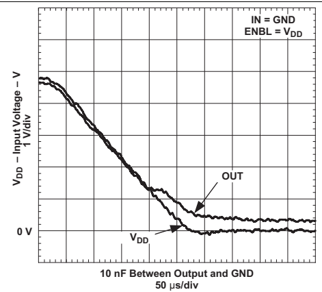
Figure 20. Output Behavior vs V_{DD} (UCC27321-Q1)
