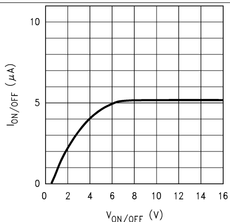
Figure 31. \text{ON}/\overline{\text{OFF}} Pin Current vs V_{\text{ON/OFF}}
