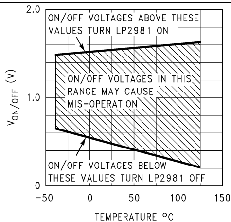
Figure 32. \text{ON}/\overline{\text{OFF}} Threshold vs Temperature
