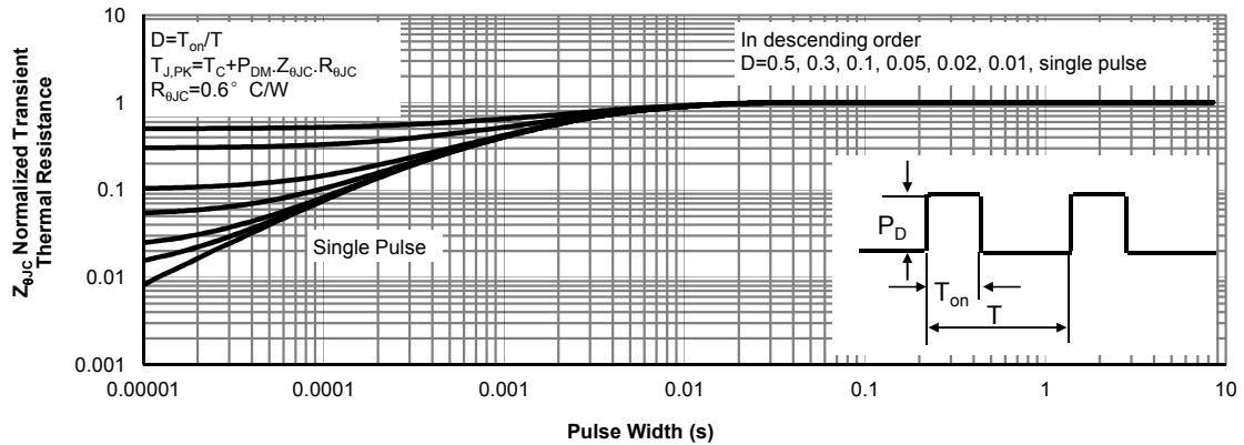
Figure 16: Normalized Maximum Transient Thermal Impedance for AOT(B)15S65L (Note F)
