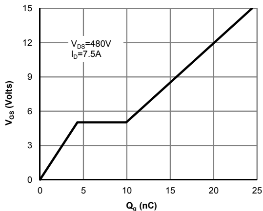
Figure 8: Gate-Charge Characteristics
