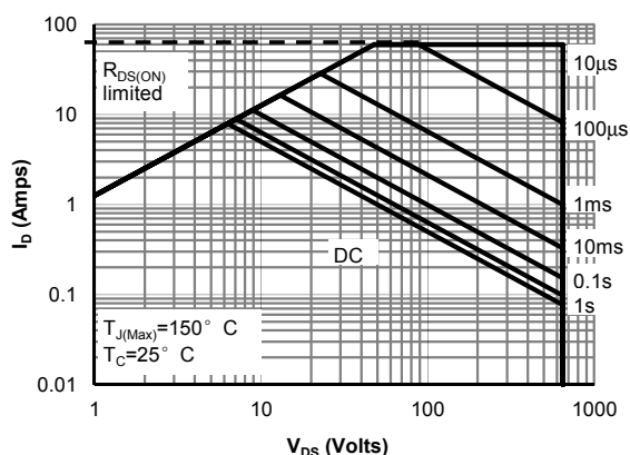
Figure 12: Maximum Forward Biased Safe Operating Area for AOTF15S65 (Note F)
