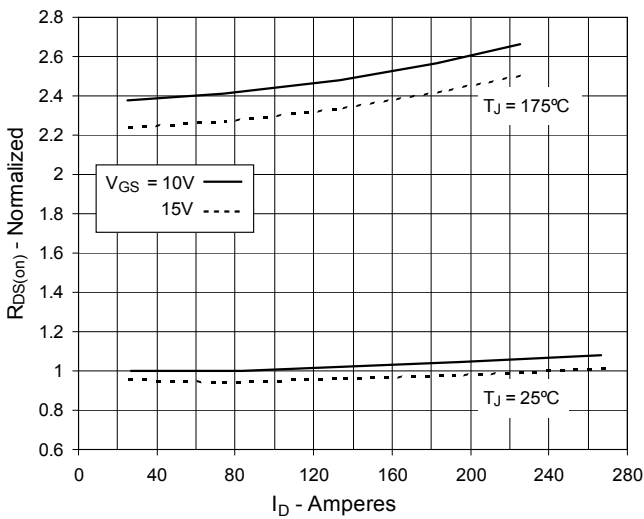
Fig. 5. R_{DS(on)} Normalized to I_D = 90\text{A} Value vs. Drain Current
