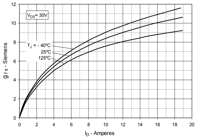
Fig. 10. Transconductance
