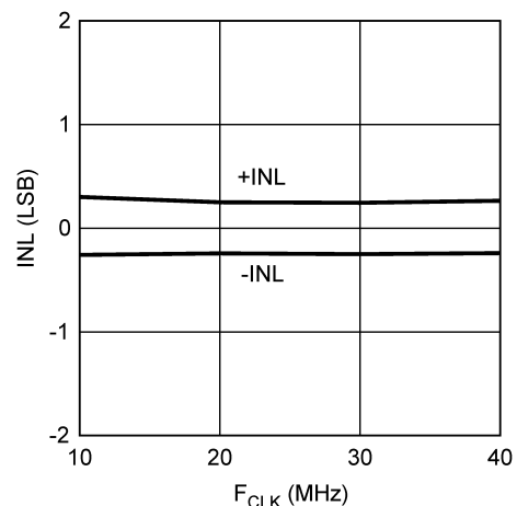
Figure 9. INL vs. f_{CLK}
