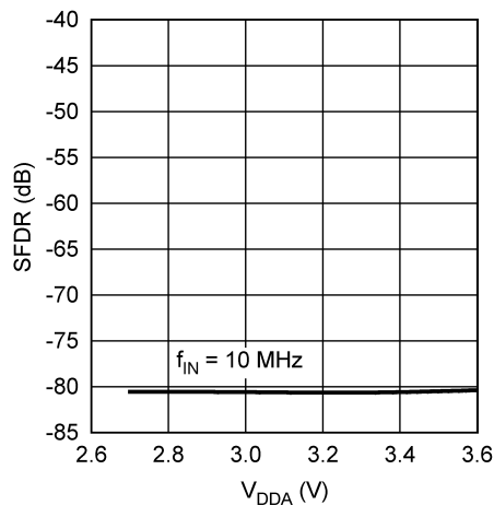
Figure 32. SFDR vs. V_{DDA}
