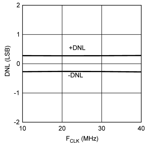
Figure 5. DNL vs. f_{CLK}
