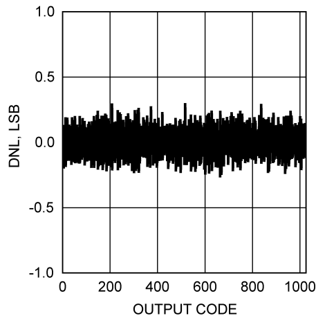
Figure 4. DNL
