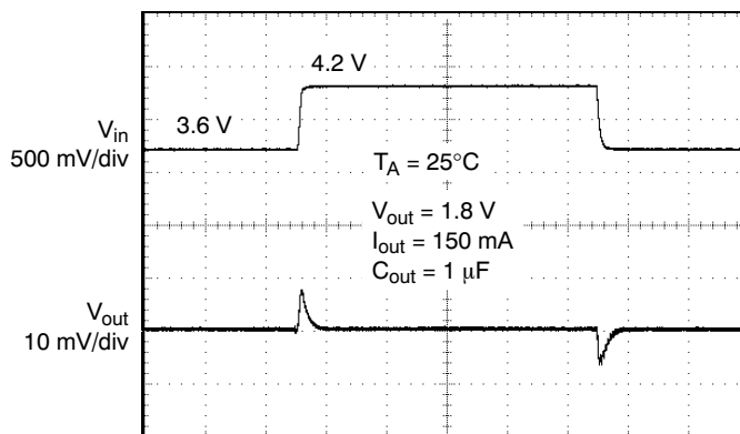
Figure 21. Line Transient
