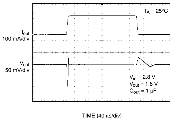
Figure 22. Load Transient
