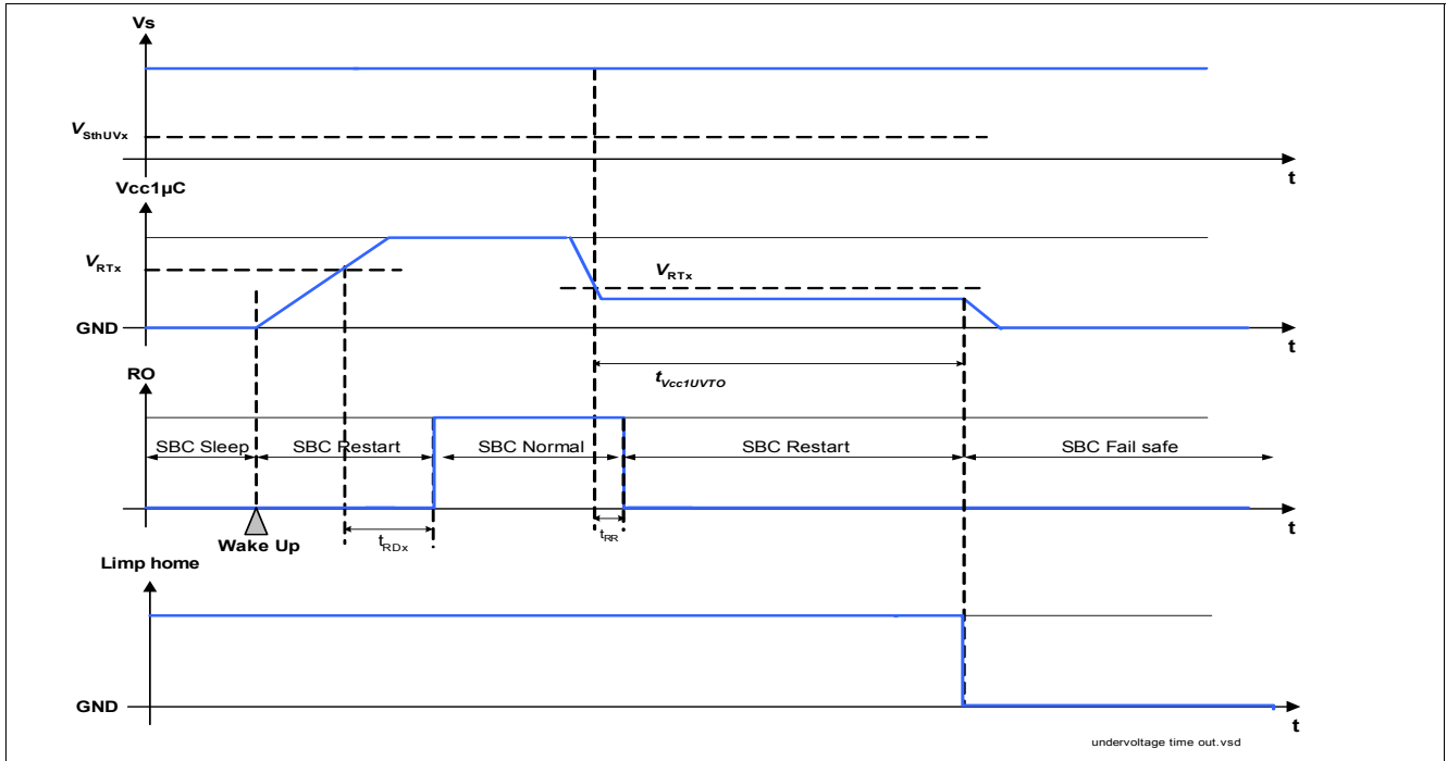
Figure 36 V cc1µC undervoltage time-out timing
