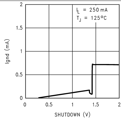
Figure 36. I_{GND} vs Shutdown
