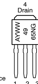
1 Gate 2 Drain 3 Source
