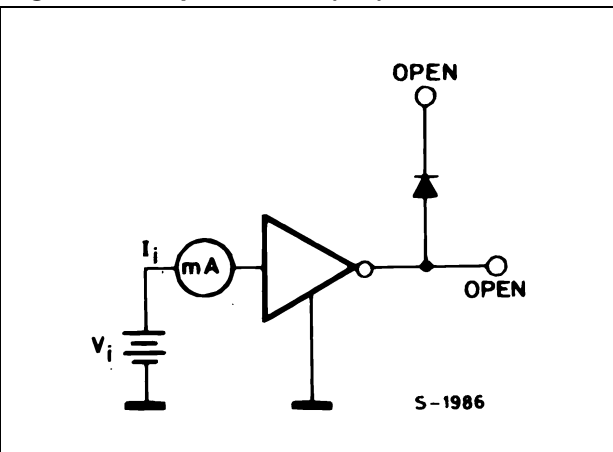
Figure 8. Input voltage
