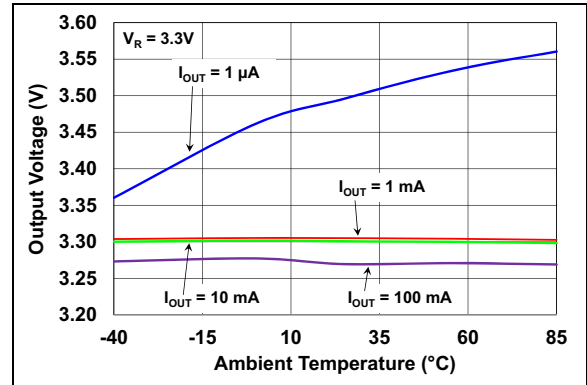
FIGURE 2-35: Output Voltage vs. Ambient Temperature.
