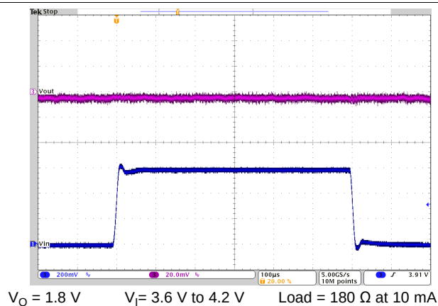
Figure 4-33. Line Transient Response LDO1
