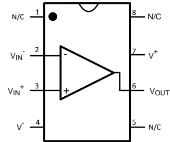
Figure 3. 8-Pin SOIC (Top View) See Package Number D0008A
