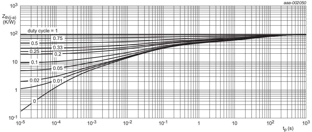
FR4 PCB, mounting pad for drain 6 \text{ cm}^2
