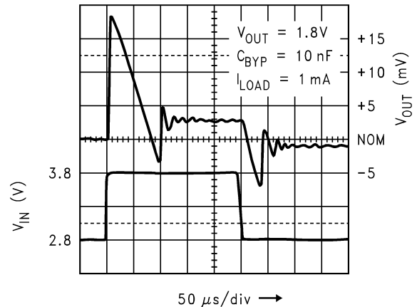
Figure 28. Line Transient
