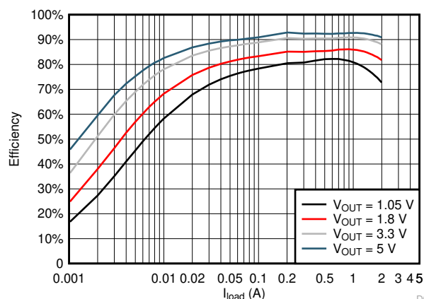
TPS562201 Efficiency
