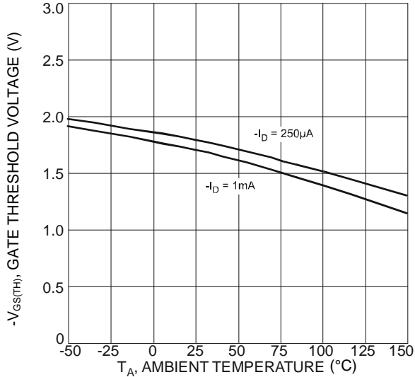
Fig. 10 Gate Threshold Voltage vs. Ambient Temperature
