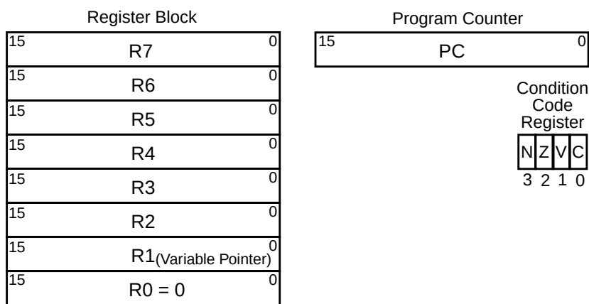
Figure 6-19. Programmer’s Model
