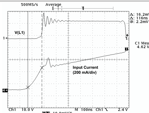
Figure 2. Low-Power-Mode Current
