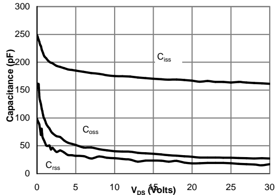
Figure 8: Capacitance Characteristics
