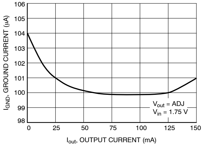
Figure 20. Ground Current vs. Output Current
