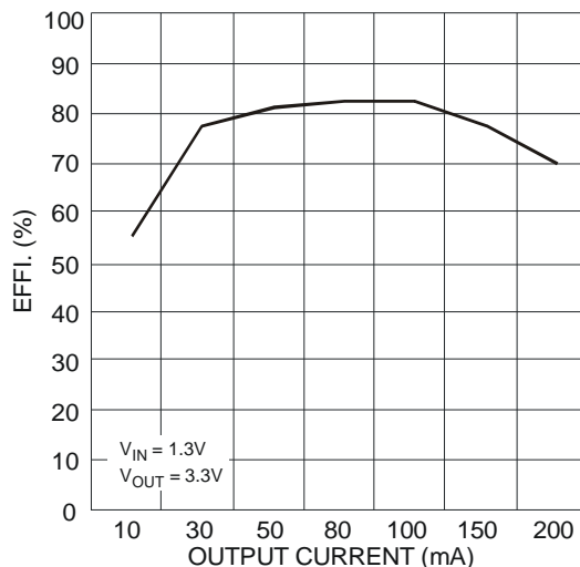
Fig. 11 EFFI. vs. Output Current
